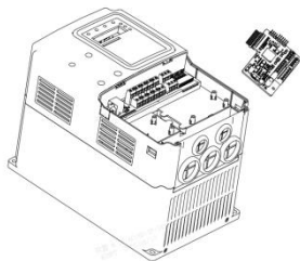
Figure 2-3 Installation diagram of Sin/Cos encoder PG card
